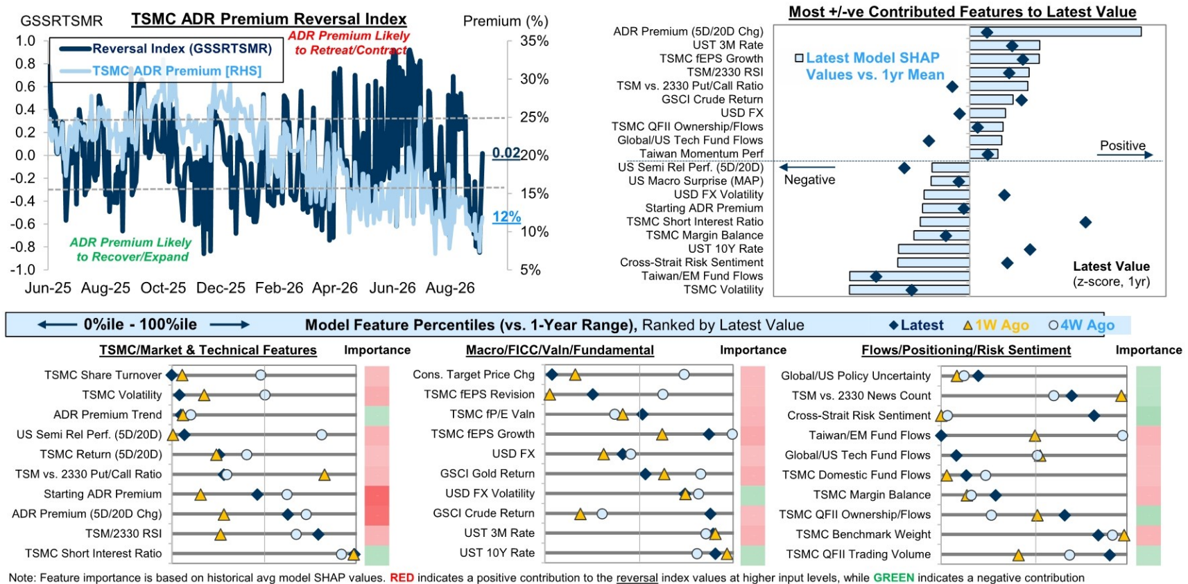
Exhibit 47: TSMC ADR Premium Reversal Index (GSSRTSMR) and the key feature contributors to its latest reading
